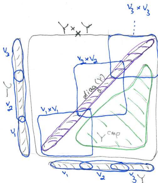
FIGURE 10. An illustration of step 1 in the proof of Theorem 16.4.33: the étale case.
