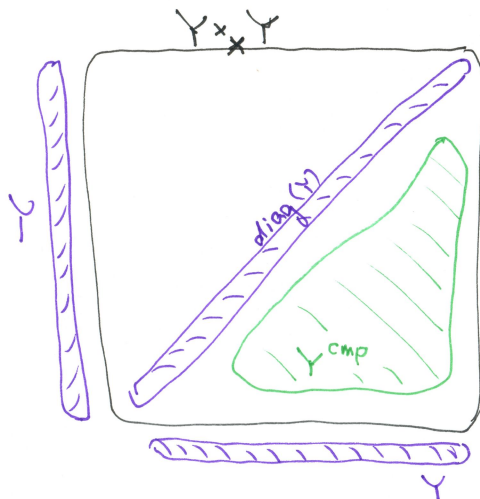
FIGURE 10. An illustration of step 1 in the proof of Theorem 16.4.33: the étale case.
