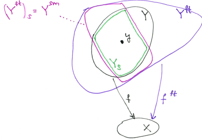
FIGURE 9. An illustration of the proof of Theorem 16.4.9. The original essentially smooth map is f : Y \rightarrow X . It is extended to a finite type map f^{\text{ft}} : Y^{\text{ft}} \rightarrow X , with an EFT embedding Y \subseteq Y^{\text{ft}} . The open subscheme Y^{\text{sm}} \subseteq Y^{\text{ft}} is smooth over X . The embedding Y_s \subseteq Y is open, and the embedding Y_s \subseteq Y^{\text{sm}} is EFT.
