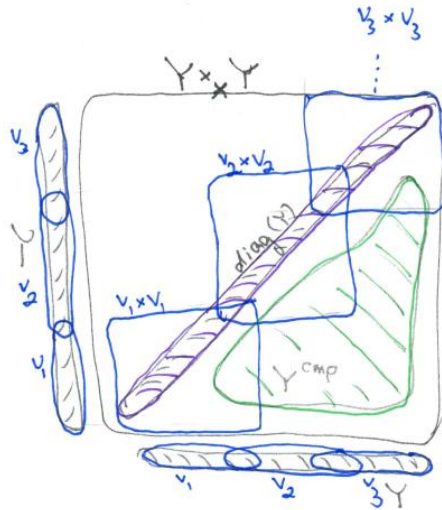
FIGURE 11. A geometric depiction of step 3 in the proof of Theorem 15.5.34: there is a covering Y = \bigcup_i V_i by affine open sets, each of them a localization of an étale X -scheme.
