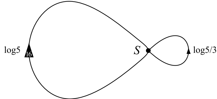
FIGURE 4. The graph associated with the substitution scheme on the square S . The large arrow stands for 16 distinct loops of length \log 5 .
