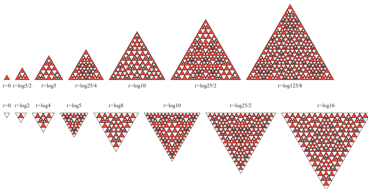
FIGURE 6. The patches F_t(U) and F_t(D) for the first values of t for which the patches contain tiles of unit volume.
