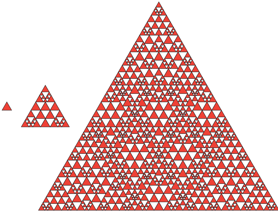
FIGURE 9. The patches F_0(U) , F_{1.\log 5}(U) and F_{2.\log 5}(U) , the first three elements of the nested sequence of patches that define a stationary tiling.
