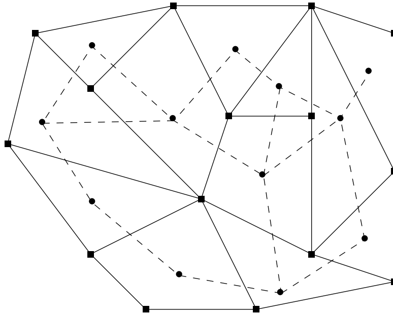
FIGURE 2. A planar graph (vertices are squares, edges are solid lines) and its dual (vertices are disks, edges are dashed lines).
