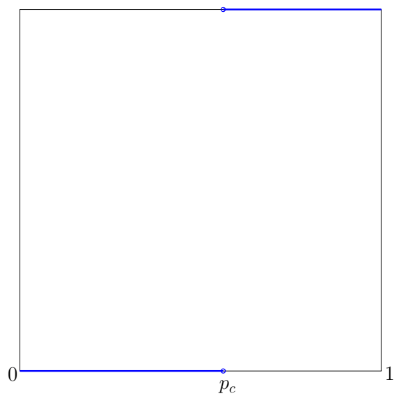
FIGURE 1. The quite boring graph of \Theta_G
