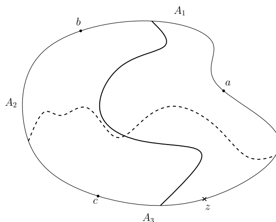
FIGURE 18. The possibilities when z \in A_3 , which cannot occur together.
