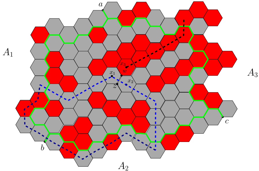
FIGURE 17. Proof of Lemma 10.5.
