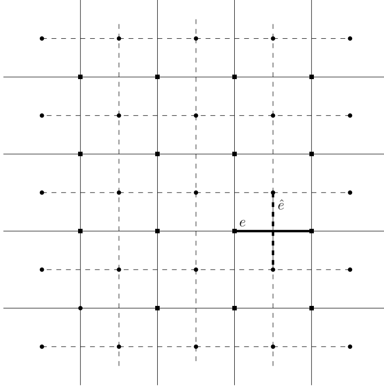
FIGURE 3. \mathbb{Z}^2 and its dual.
