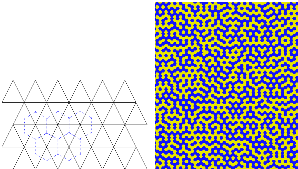
FIGURE 10. Left: The triangular lattice \mathbb{T} and part of its dual lattice, the hexagonal (or honeycomb) lattice \mathbb{H} . Right: Percolation on the faces of \mathbb{H} = site percolation on \mathbb{T} .
