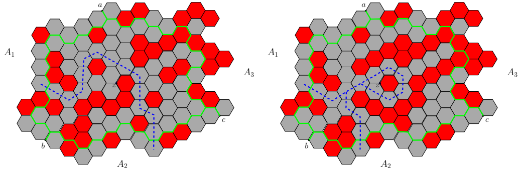
FIGURE 16. Left: The event S^3(z) . Right: S^3(z) does not hold, because the path is not simple.
