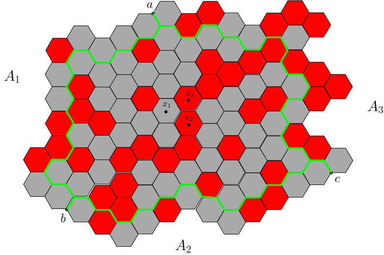
FIGURE 14. A nice domain with three marked points on the boundary, and three adjacent hexagons x_1, x_2, x_3 inside. Note the event B_1 \circ R_2 \circ R_3 .
