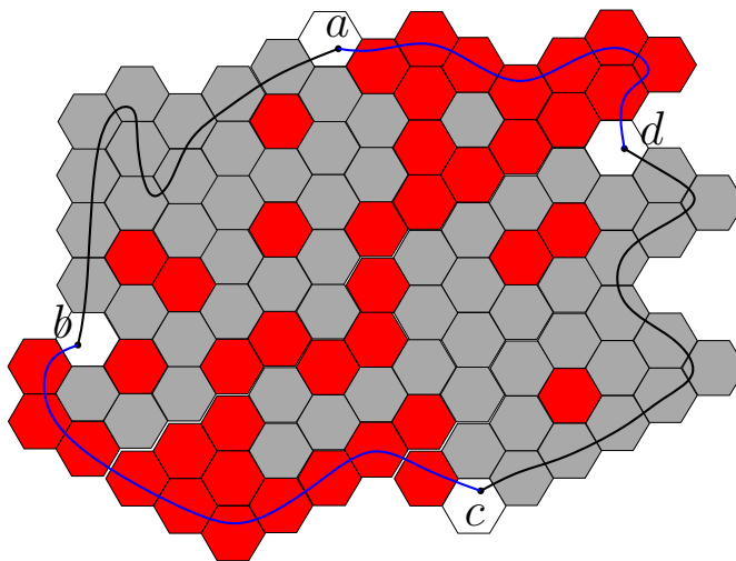
FIGURE 12. A domain D with four marked points a, b, c, d . The hexagonal lattice \mathbb{H} is drawn, and is colored according to some configuration \omega . Can you find the red crossing from (b, c) to (d, a) ?
