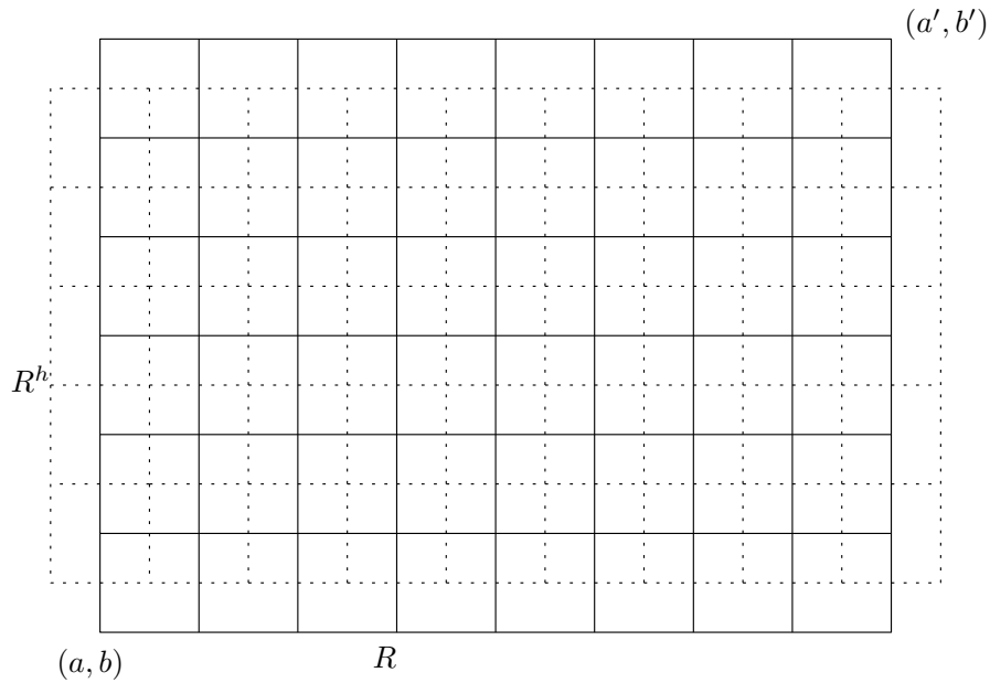
FIGURE 7. A rectangle in \mathbb{Z}^2 and its dual.
