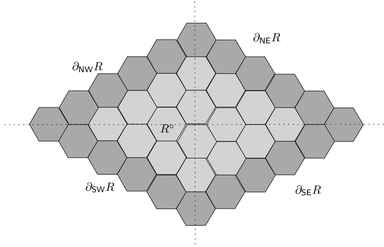
FIGURE 11. The rhombus R ( n = 6 ).
