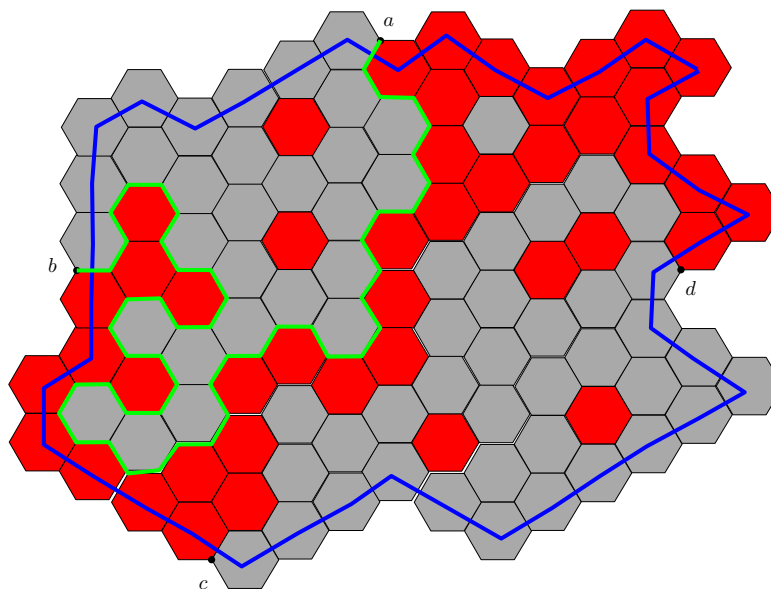
FIGURE 13. A nice domain D . The path tracing the boundary is marked in blue. Four points in \mathbb{C}_\delta dividing the boundary into four parts are shown. The exploration path from b is marked in green.
