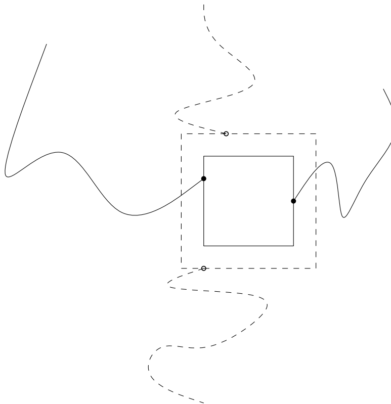
FIGURE 9. The event A from Zhang's argument.
