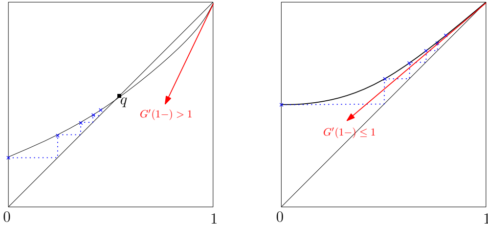
FIGURE 5. The two possibilities for G'(1-) . The blue dotted line and crosses show how the iterates G^{(n)}(0) advance toward the minimal solution of G(z) = z .
