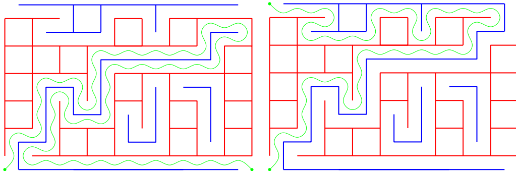
FIGURE 8. Two possibilities for exploration of the component of \partial_W R .
