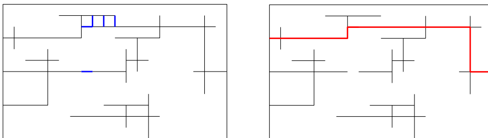
FIGURE 6. Two examples of configurations \omega with edges that are pivotal in \omega for the event of crossing the rectangle from left to right. On the left, blue edges are closed, and are all pivotal. On the right, red edges are all open, and are all pivotal.
