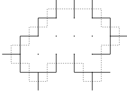
FIGURE 4. A minimal cut-set and its dual self-avoiding polygon.
