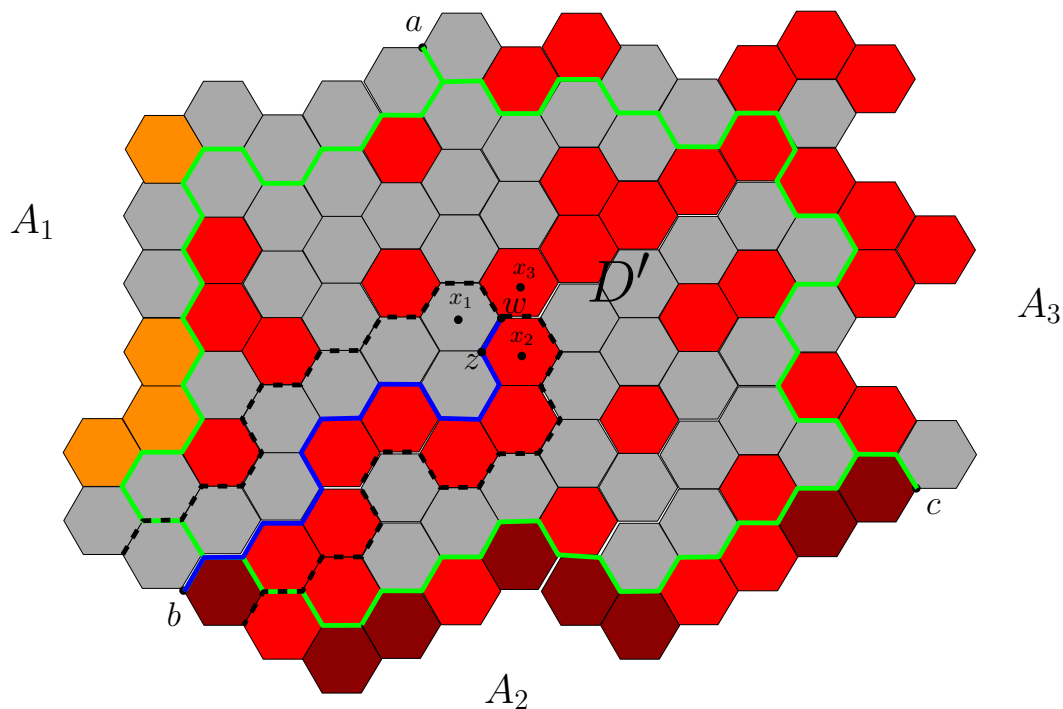
FIGURE 15. The proof of (10.2). The blue line is the interface \gamma , which only explores those hexagons in the dotted black boundary. What is left over is D' .
